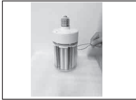
Step 2: Insert the safety cable through the safety cable slot on the side of the plastic base.
